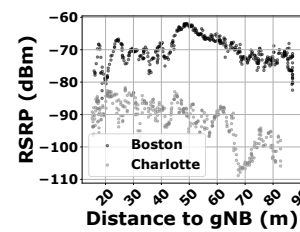
Figure 1: RSRP vs. Distance for two gNBs in Boston and Charlotte.
